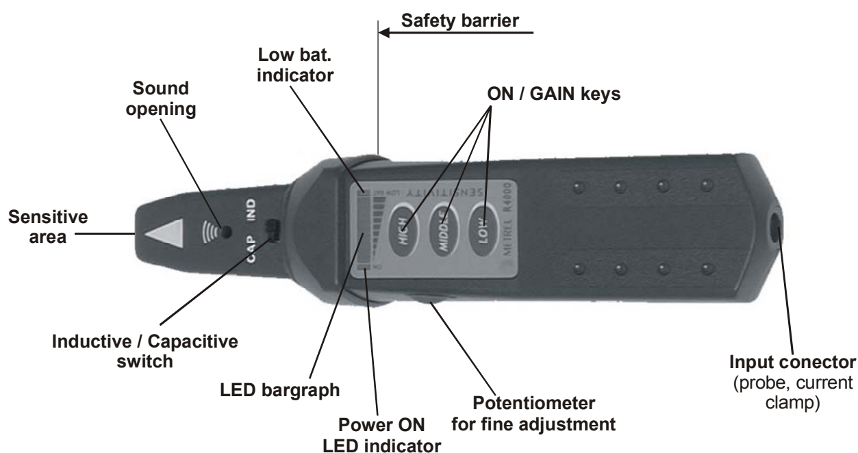
Fig. 2. Receiver R10K
