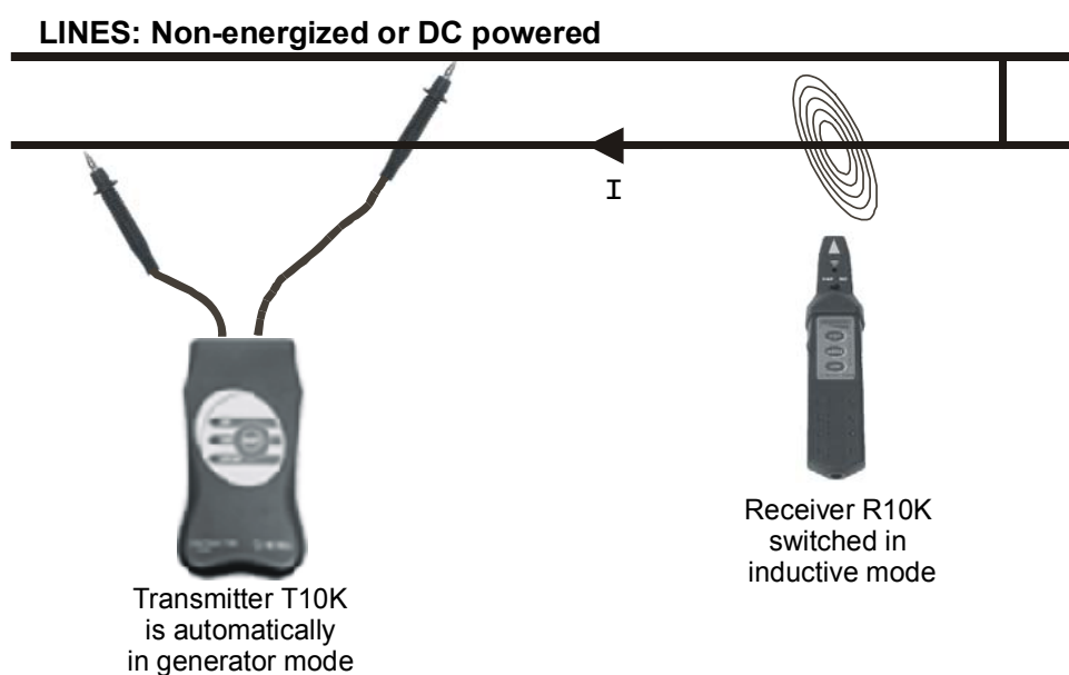
Fig. 7. Injection of test current into tested loop
