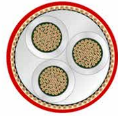
➤ Belted medium voltage cable with common shield, 3 conductors, faults between core and core and shield, fault location difficult due to multiple path, core - core likely
