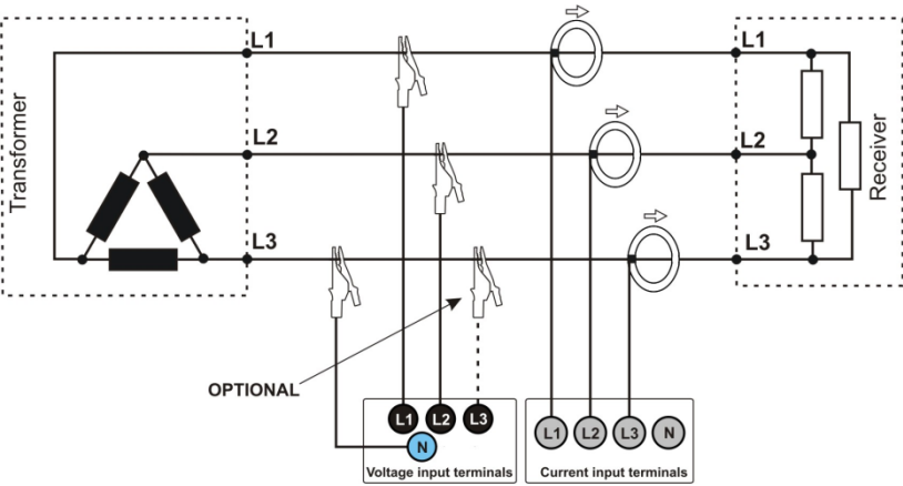
Fig. 9. Wiring diagram – 3-phase delta.
