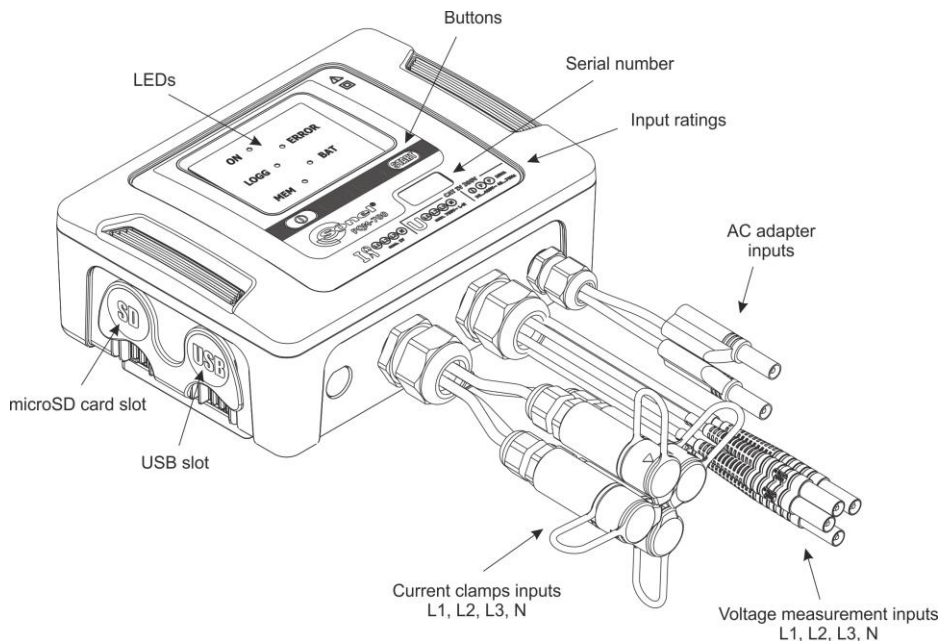
Fig. 1. Power Quality Analyzer PQM-700. General view.
