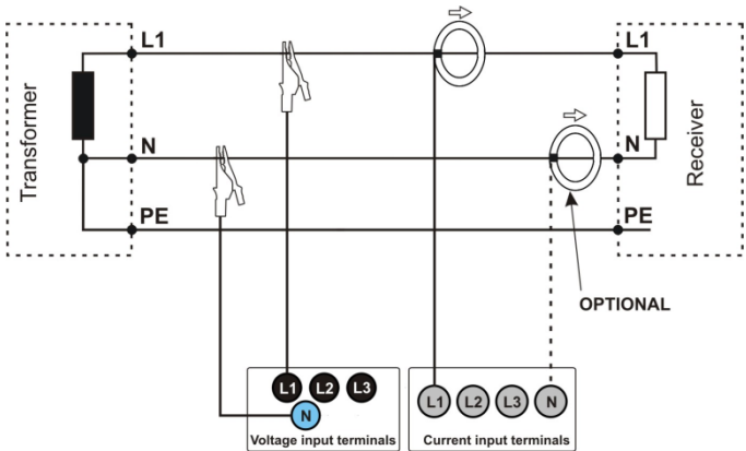
Fig. 5. Wiring diagram – single phase.
