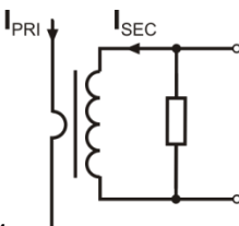
Fig. 16. Current transformer clamp with voltage output.
