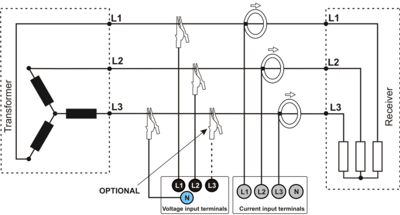
Fig. 8. Wiring diagram – 3-phase wye without neutral conductor.
